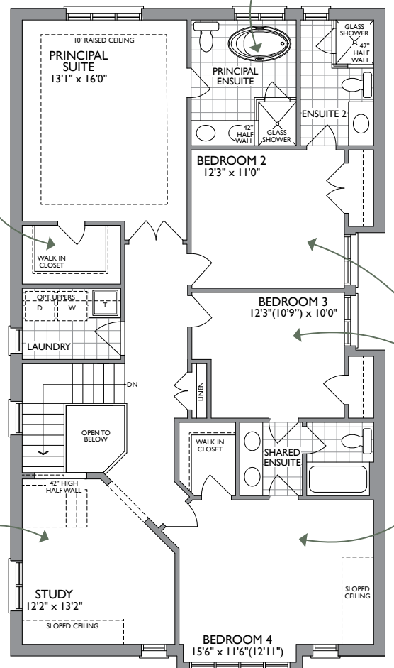
SECOND LEVEL
