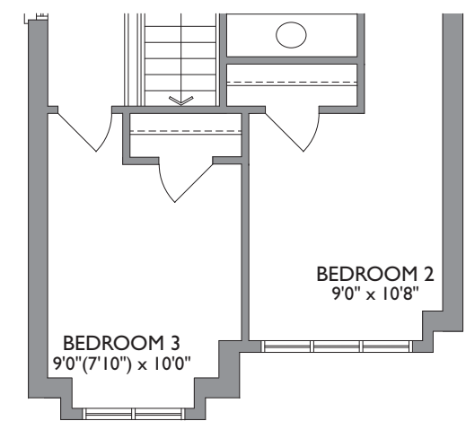
SECOND FLOOR ELEV. AB
